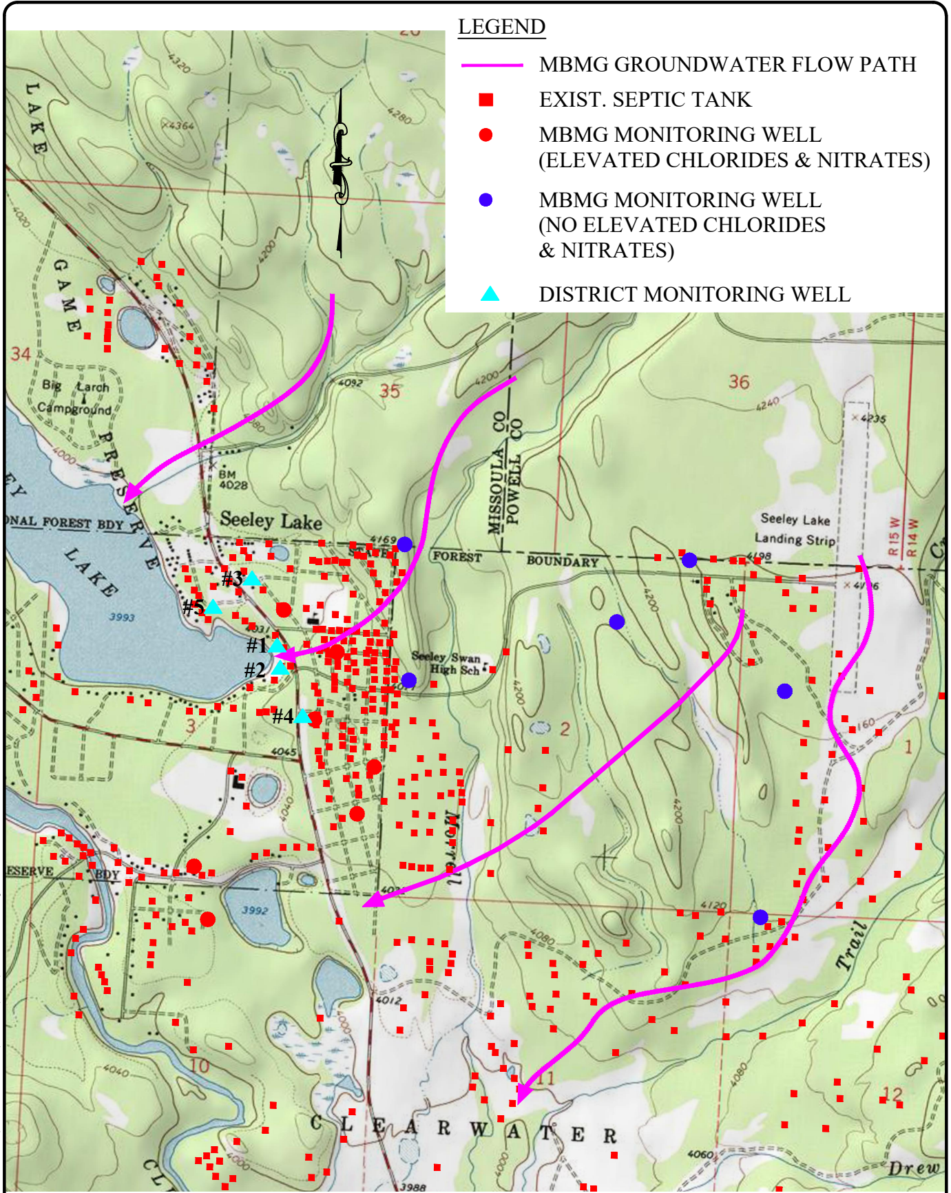
Figure 3-1 GROUNDWATER FLOW PATHS, MONITORING WELL LOCATIONS, AND SEPTIC LOCATIONS
